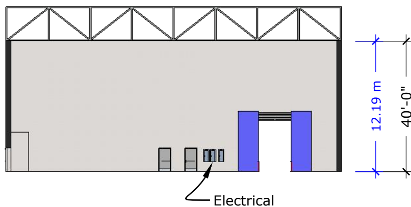
S ELEV SOUTH scale: 1" = 30' [1:360]
