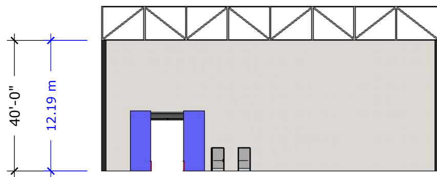
N ELEV NORTH scale: 1" = 30' [1:360]
