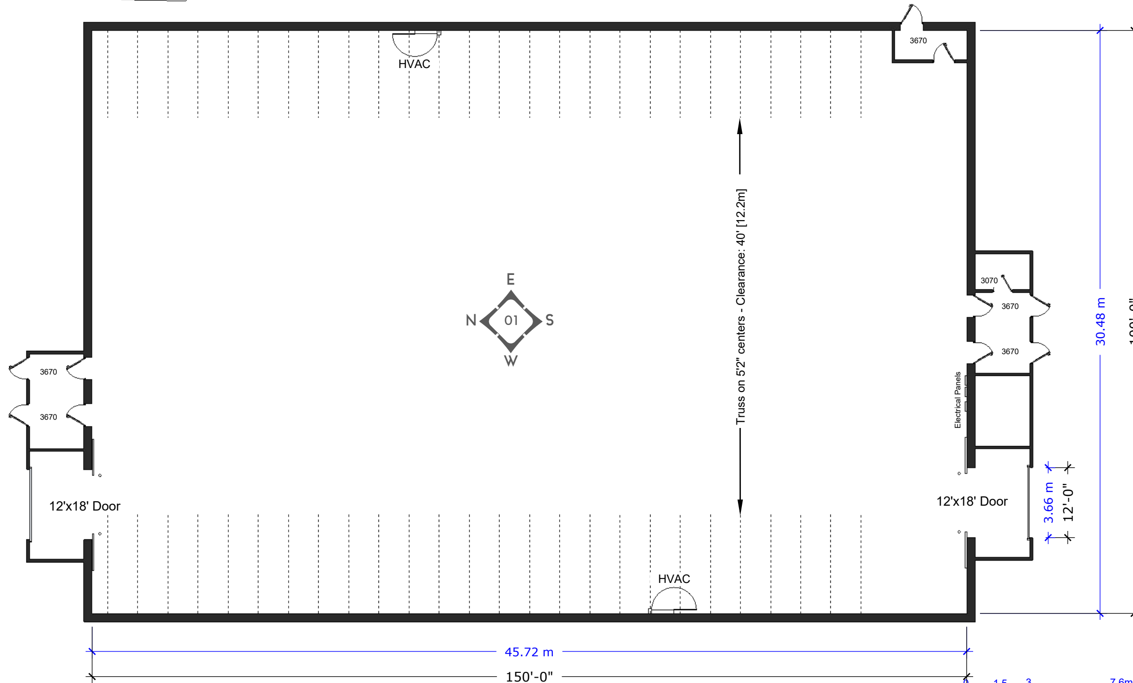
S4 STAGE 4 - PLAN scale: 1/16" = 1' [1:192]
