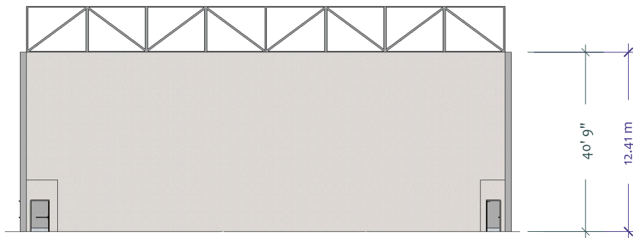
3 :: South Wall scale: 1" = 30' (1:360)
